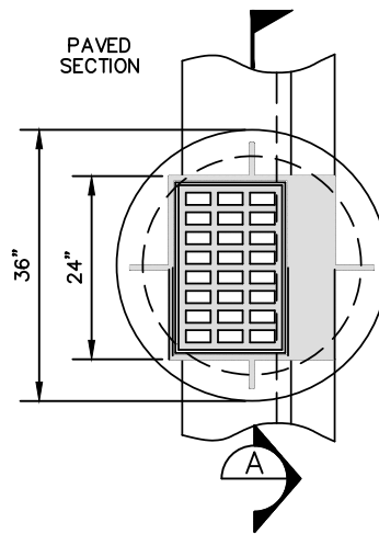
PLAN VIEW
