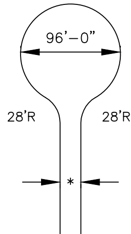
96' CUL-DE-SAC TURNAROUND
