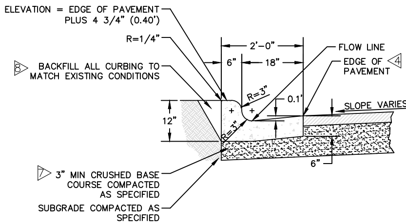
STANDARD "CATCH" TYPE CURB
